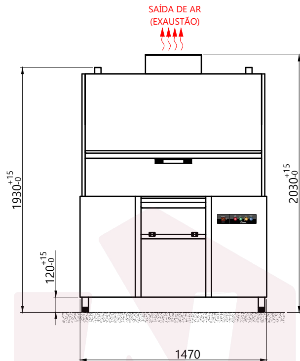
VISTA FRONTAL
