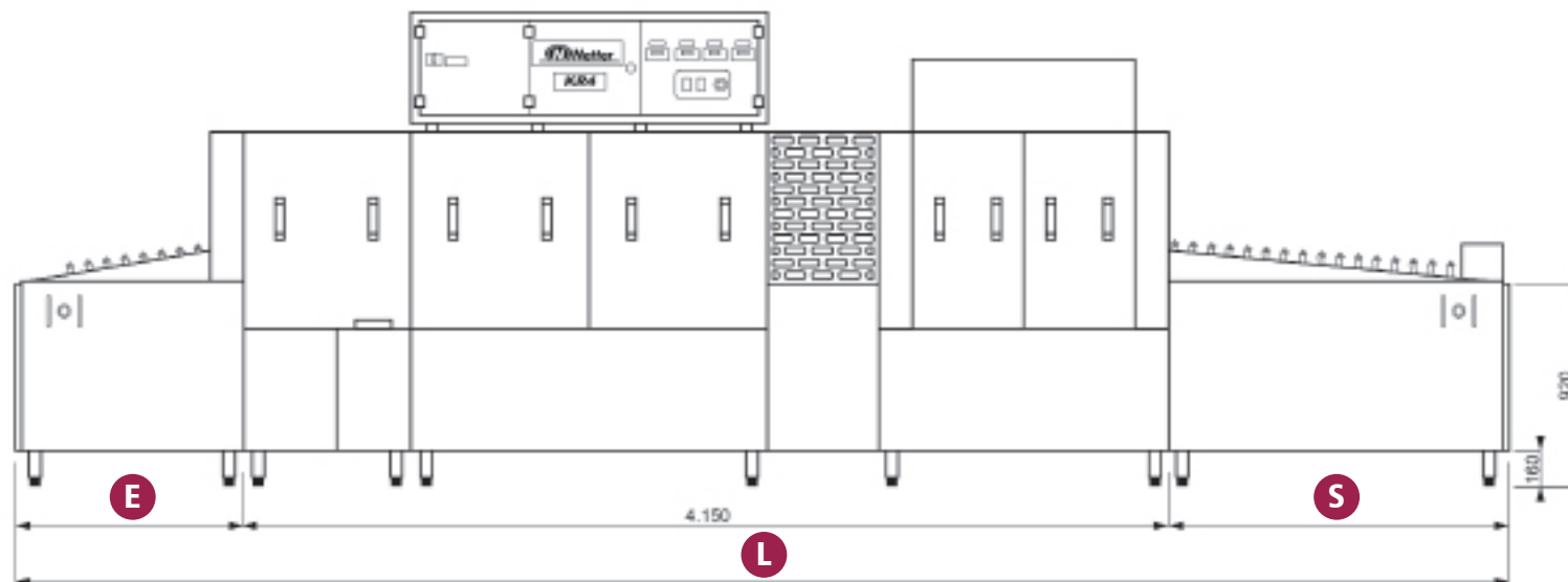
VISTA FRONTAL
