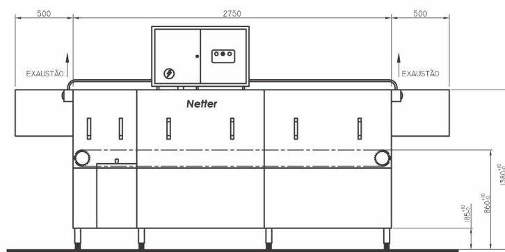
VISTA FRONTAL
