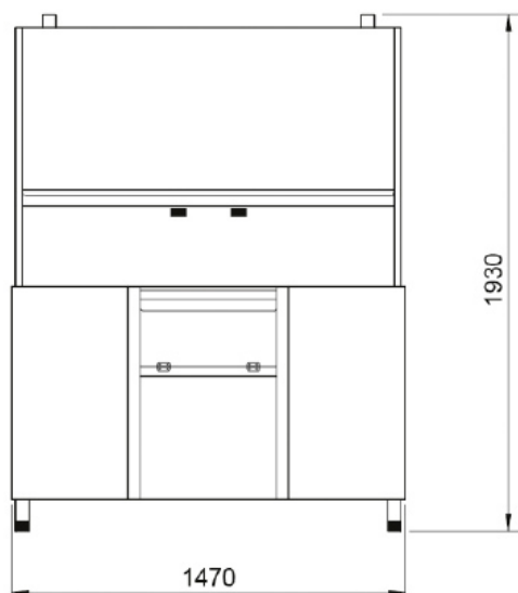
VISTA FRONTAL
